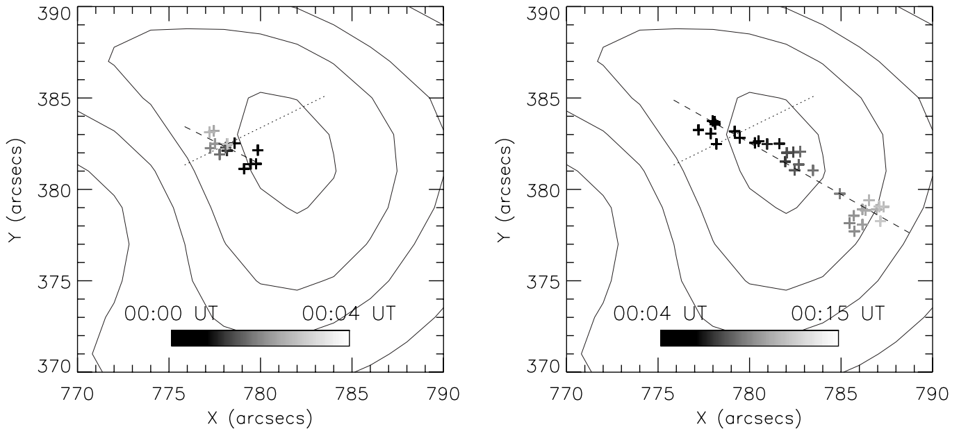
FIG. 4.—Loop-top centroids ( crosses ) overlaid on the loop-top region contours of that 12–25 keV image of the 2002 April 14–15 flare at 00:01:00 UT shown in Fig. 2. The left and right panels show the centroids moving downward before 00:04 UT and upward after 00:04 UT, respectively. In both panels, the dotted lines represent the radial direction, while the dashed lines, which are from a linear fit to the centroid locations, represents the direction of motion. The angles between the radial direction and the direction of motion are 53^\circ ( left ) and 56^\circ ( right ). [See the electronic edition of the Journal for a color version of this figure.]
