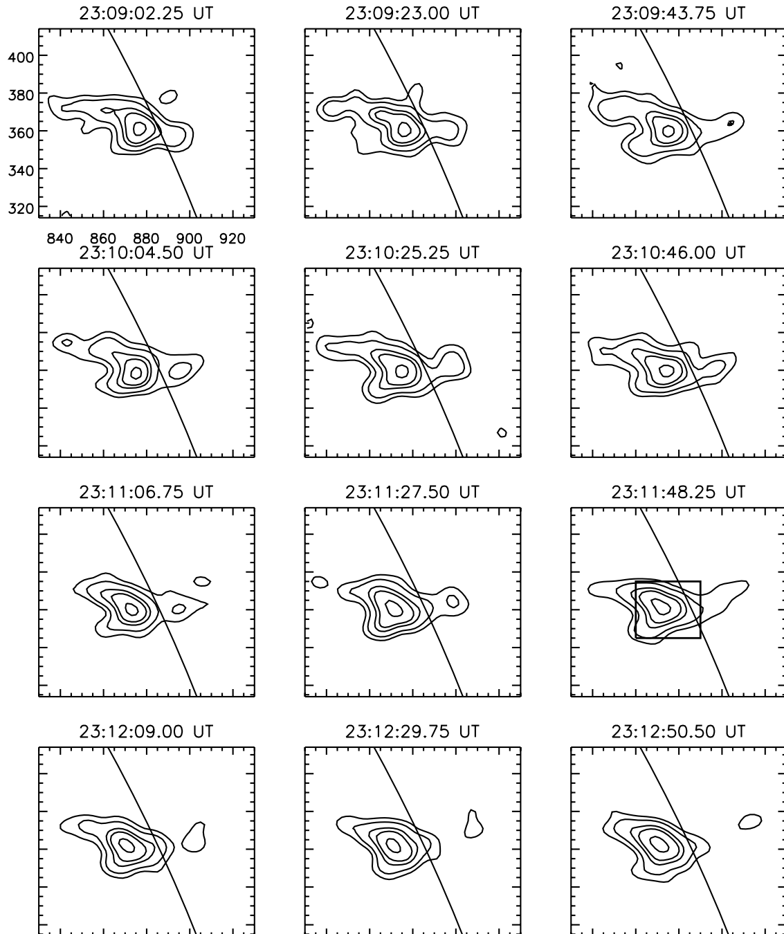
FIG. 5.—Time sequence of 10–25 keV RHESSI images for the 2002 April 15 flare. The imaging parameters are the same as those used in Fig. 2. The contour levels are 15%, 25%, 45%, 60%, and 90% of the peak flux in each image. The box in the image at 23:11:48.25 UT delineates the size of the image view in Fig. 7. The solid line denotes the solar limb.
