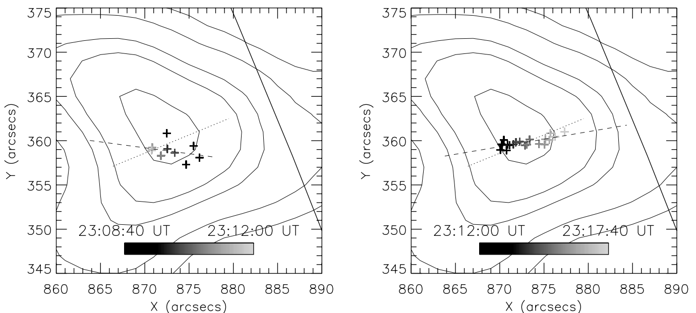
FIG. 7.—Loop-top centroids (crosses) overlaid on the loop-top region of the 10–25 keV image of the 2002 April 15 flare at 23:11:48.25 UT shown in Fig. 5. The other aspects of the figure are the same as for Fig. 4. The angles between the radial direction and the direction of motion are 30^\circ (left) and 13^\circ (right). [See the electronic edition of the Journal for a color version of this figure.]
