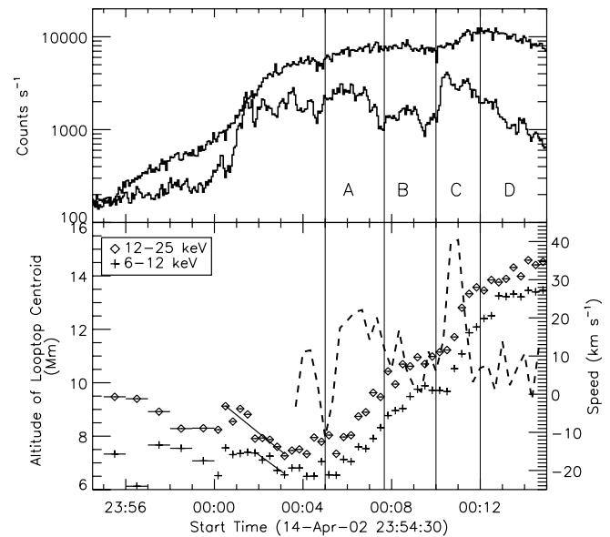
FIG. 3.— Top : Light curves in two energy bands ( upper curve , 6–12 keV rate \times 0.1 ; lower curve , 25–50 keV rate \times 1.0 ) for the 2002 April 14–15 flare. Bottom : Altitude of the loop-top centroid within the 60% contour for the images in the 6–12 ( crosses ) and 12–25 keV ( diamonds ) bands. The horizontal bars on each point represents the integration time of the corresponding image. The solid lines show linear fits to the altitudes vs. time for two time ranges and two energy bands. The dashed line represents the apparent velocity of the loop top, determined by taking the time derivative of the 12–25 keV altitude curve after 00:03:50 UT.
