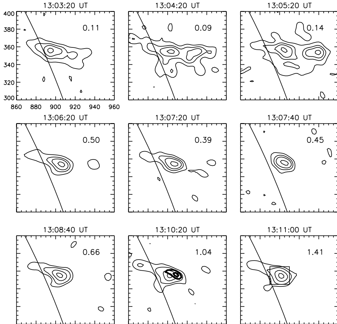
FIG. 8.— RHESSI 12–25 keV images for the 2002 April 16 flare. The imaging parameters are the same as those used in Fig. 2. The integration time of the images was 1 minute before and 20 s after 13:07:20 UT. For the top two rows, the contour levels are 20%, 40%, 60%, and 90% of the peak flux in each image. For the bottom row, the contour levels are 15%, 30%, 60% and 90%. A RHESSI 25–50 keV image at 13:10:20 UT (contour levels showing 60% and 90% of the peak flux) is plotted on the 12–25 keV image at the same time. The number on each image is the peak flux ( \text{cm}^{-2} \text{s}^{-1} \text{arcsec}^{-2} ) in 2'' pixels. The box in the image at 13:11:00 UT delineates the size of the image view in Fig. 10.
