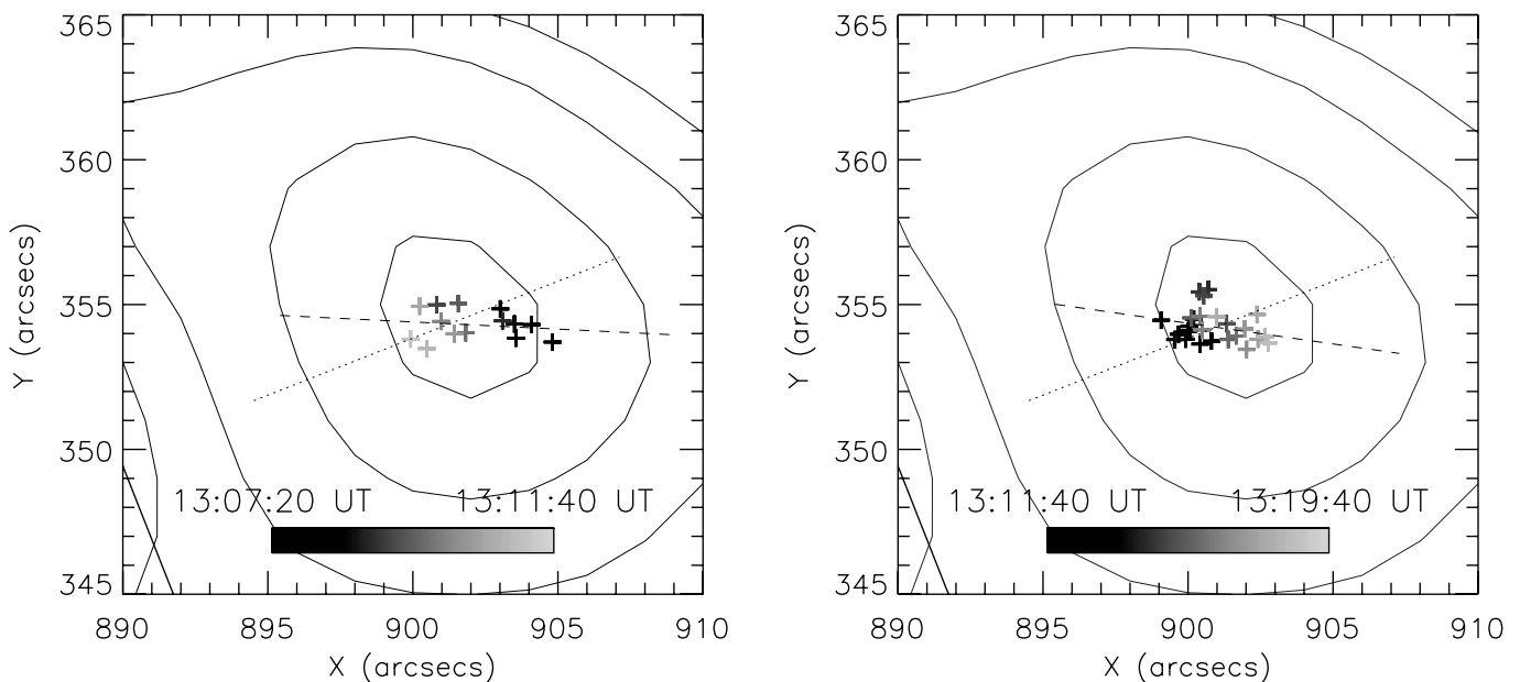
FIG. 10.—Loop-top centroids ( crosses ) overlaid on the loop-top region of the 12–25 keV image of the 2002 April 16 flare at 13:11:00 UT in Fig. 8. The other aspects of the figure are the same as in Fig. 4. The angles between the radial direction and the direction of motion are 24° ( left ) and 30° ( right ). [See the electronic edition of the Journal for a color version of this figure.]
