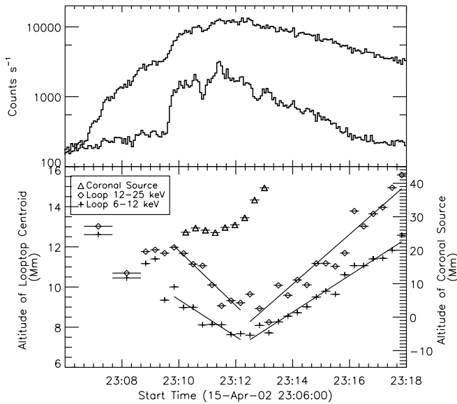
FIG. 6.— Top : Light curves in two energy bands ( upper curve , 6–12 keV rate \times 0.5 ; lower curve , 25–50 keV rate \times 1.0 ) of the 2002 April 15 flare. Bottom : Altitude of the loop-top centroid obtained using the 60% contour for the images in the 6–12 (crosses) and 12–25 keV (diamonds) bands. The triangles show the altitude of the coronal source above the flare loop. The horizontal bars on each point represents the integration time of the corresponding image. The lines show linear fits to the altitudes vs. time for two time ranges and two energy bands.
