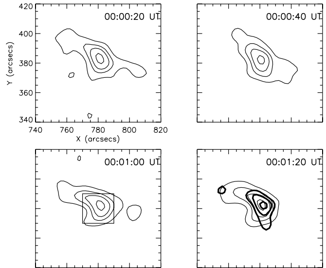
FIG. 2.—Sequence of 12–25 keV RHESSI images at the time of the impulsive rise of the 2002 April 14–15 flare (see Fig. 1, top ). The time in each box is the start time of the 20 s integration time interval ( \sim 5 RHESSI rotation periods). RHESSI grids 3–9 were used, giving an angular resolution \sim 7'' . The contour levels are 20%, 40%, 60%, and 90% of the peak flux in each image. The box in the image at 00:01:00 UT delineates the size of the image in Fig. 4. The thick contours overlaid on the image at 01:20 UT are for the 25–50 keV band at 40%, 60%, and 90% of the peak flux. Start times of images are indicated. The accumulation time of each images is 20 s.
