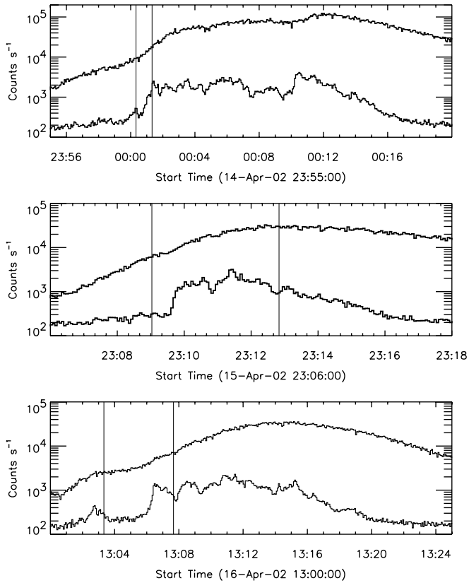
FIG. 1.— RHESSI light curves of the three flares, 2002 April 14–15 ( top ), 15 ( middle ), and 16 ( bottom ). The energy bands in each panel are 6–12 ( upper curve ) and 25–50 keV ( lower curve ). The solid lines in each panel mark the time range for the images in Figs. 2, 5, and 8. The time range was selected to show the RHESSI images with the coronal source above the flare loop.
