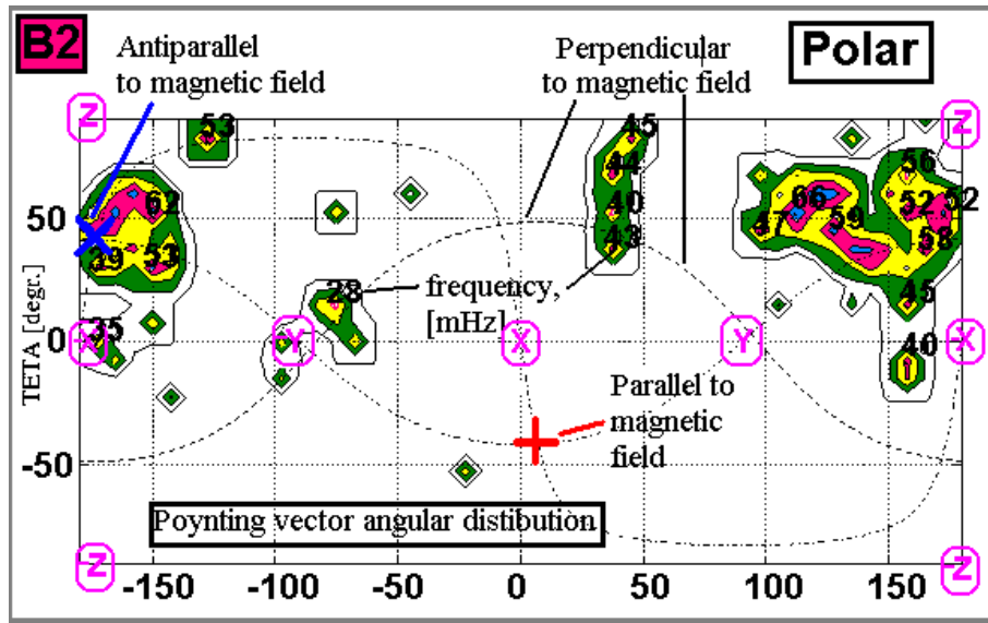
Plate B2. 07:00:00–07:01:56 UT: angular distribution of the Poynting flux in GSM coordinates from Polar; median frequency of the maxima is given in mHz (see details in text).
