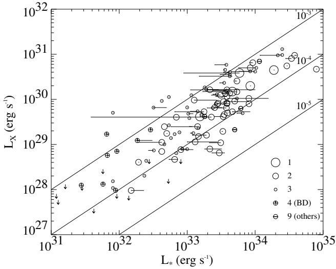
Fig. 13. X-ray luminosity L_X (based on DEM fits) vs. stellar luminosity L_* for all X-ray detected XEST sources ( Chandra sources, Herbig stars, and objects “below” the ZAMS not included), or upper limits (arrows). For multiple systems, total (“system”) luminosity L_* has been used. Symbols defining the object type are given in the lower right corner. The horizontal bars for some objects show the ranges of literature values for L_* , while the circle marks the adopted L_* .
