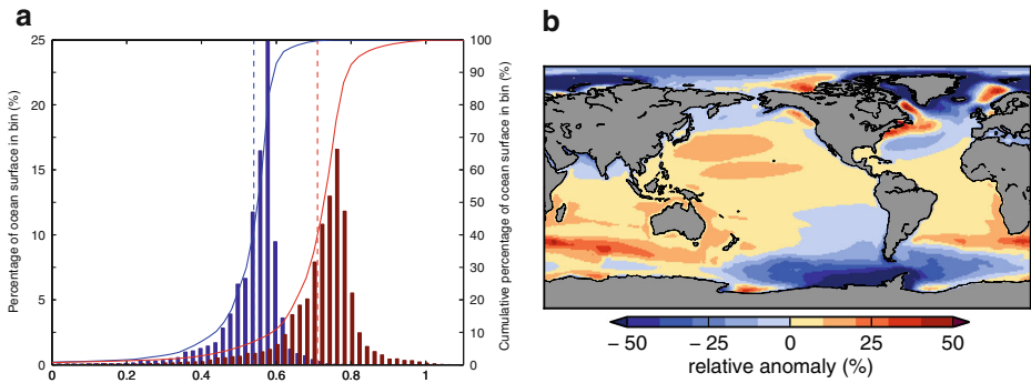
Fig. 4 a Histogram of the binned local SLC (% of the total ocean surface, left axis ); scenario A ( blue ), scenario B ( red ). Dashed lines indicate the global mean (0.54 and 0.71, respectively), solid lines the cumulative percentage ( right axis ). Bin width is 0.02 m. Percentage of ocean surface with less than 0 m SLC is 0.49% (A) and 0.37% (B), there are no values over 1.1 m. b Scenario A relative SLC anomaly w.r.t. the global mean (%) between 1986–2005 and 2081–2100
