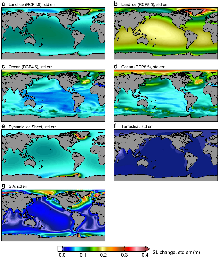
Fig. 2 Uncertainties ( 1\sigma ) of projected relative SLC patterns (m) of individual contributions over the period 1986–2005 to 2081–2100; (a) RCP4.5 glaciers + ice sheet SMB, (b) RCP8.5 glaciers + ice sheet SMB, (c) RCP4.5 global steric+dynamic topography + AL, (d) RCP8.5 global steric+dynamic topography + AL, (e) Ice sheet dynamics, (f) Groundwater depletion, (g) GIA. Global mean uncertainties in Table 1
