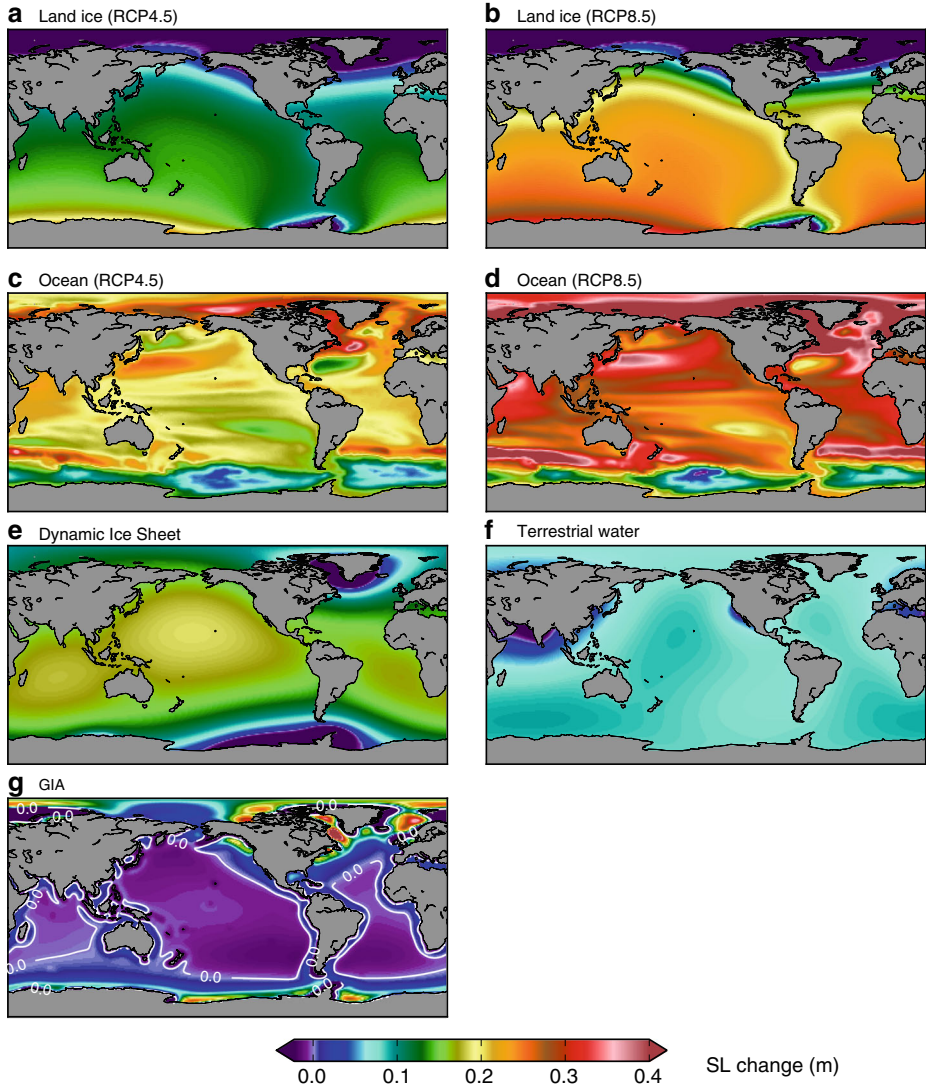
Fig. 1 Projected relative SLC patterns (m) of individual contributions over the period 1986–2005 to 2081–2100; a RCP4.5 glaciers + ice sheet SMB, b RCP8.5 glaciers + ice sheet SMB, c RCP4.5 global steric+dynamic topography + AL, d RCP8.5 global steric+dynamic topography + AL, e Ice sheet dynamics (scenario-independent), f Groundwater depletion (scenario-independent), g GIA (scenario-independent). Global mean values in Table 1
