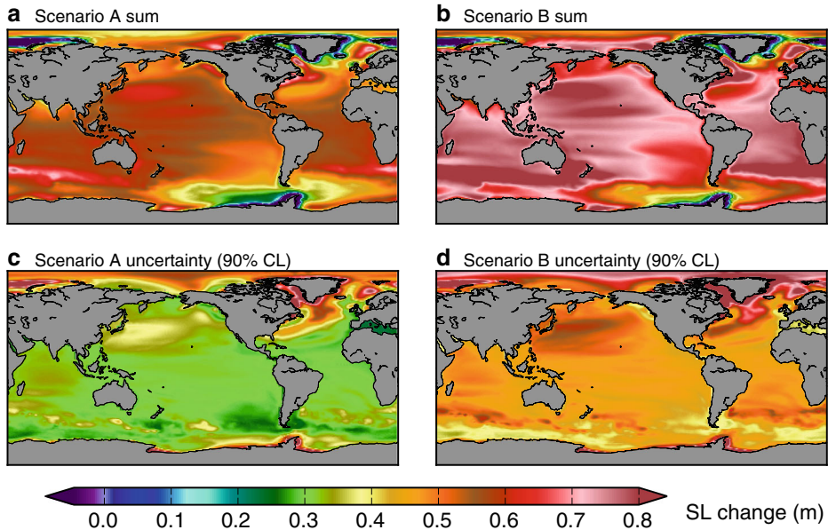
Fig. 3 Combined regional SLC patterns and uncertainties over the period from 1986–2005 to 2081–2100 for a Scenario A sum (=Fig. 1a+c+e+f+g, global mean is 0.54 m), b Scenario B sum (=Fig. 1b+d+e+f+g, global mean is 0.71 m), c Scenario A uncertainties at the 90 % confidence level (global mean is 0.32 m), d Scenario B uncertainties at the 90 % confidence level (global mean is 0.48 m)
